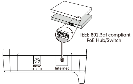
b. PoE (Power over Ethernet) Option
